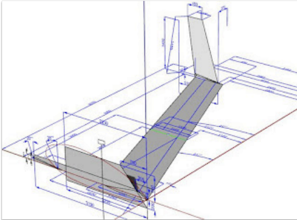
The panel model used in the VLM code.
