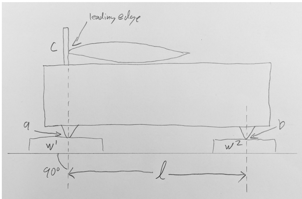
fig. 1 Diagram of build elements requiring precision.
