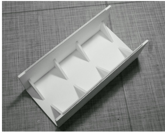
fig. 7 Hot glued dowel | fig. 8 Scale sides and leading edge stops | fig. 9 Frame side in place | fig. 10 Completed sides with triangle reinforcements
