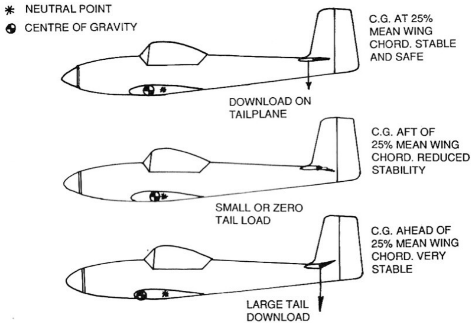
Figure 5.6 C.G. Location and stability in pitch
