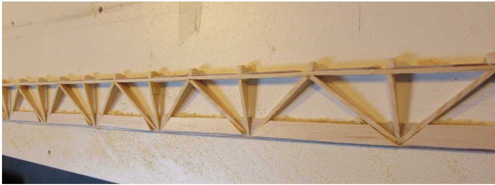
Aileron cut off, it needs reinforcement!
