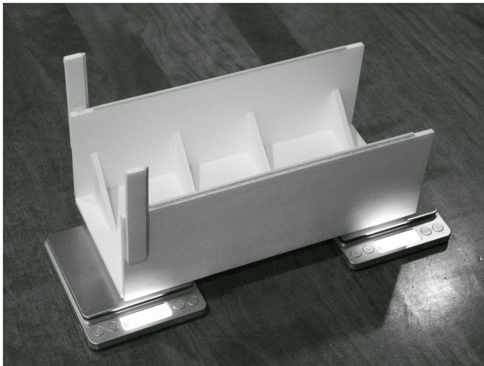
fig. 20 The completed CG frame + scales
