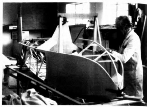
Building the modern replica of the British Falcon at Southdown Air Services. (K. Frupp)
