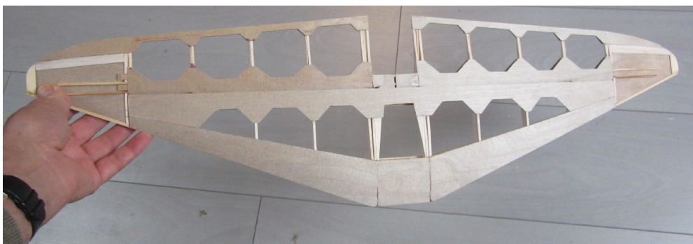
Stabiliser almost finished.
