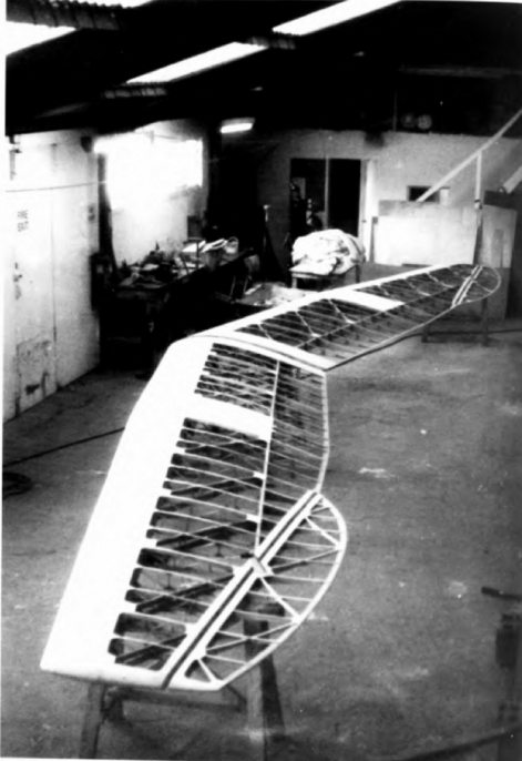
Building the modern replica of the British Falcon at Southdown Air Services. (K. Frupp)
