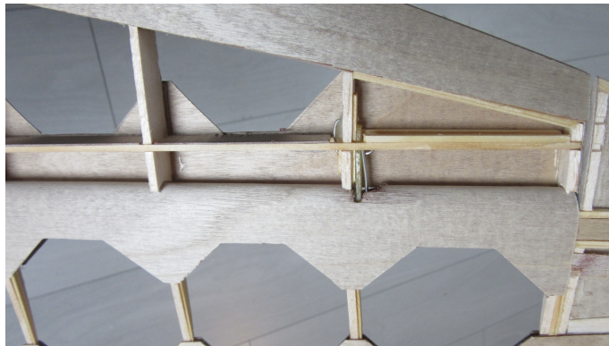
Left: stabiliser mounting strips and hinged control rod of the elevator. | Right: The hinge is in the 'locked' position. It will later be sheeted with ply.
